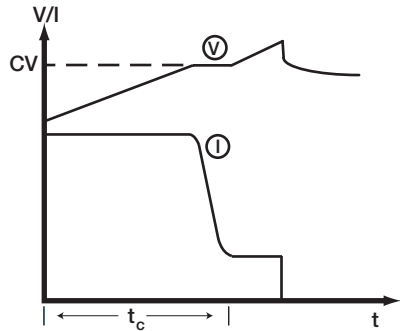
Figure 2. End of Charge Profile with Equalize
