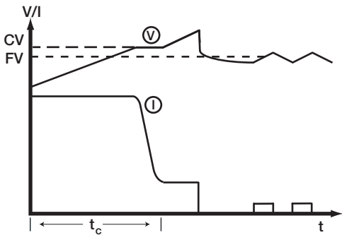
Figure 4. Float Profile with Equalize
